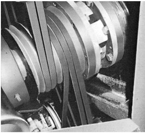
Marine Engine (TSCHAN® Coupling S )
