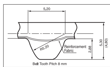
Standard Belt Width
