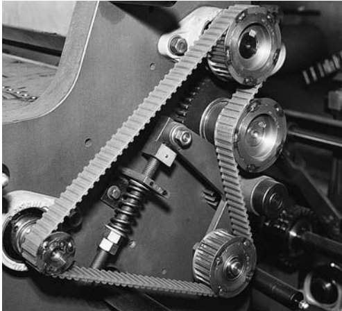
Packaging Machine (Polyurethane Double Timing Belt)
