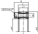
STL - 20S - 20 - 47 Outer Diameter Inner Diameter (Shaft Diameter) Model Number Starlock
