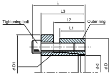
STL - 21S - 19 - 47 Outer Diameter Inner Diameter (Shaft Diameter) Model Number Starlock
