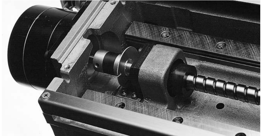
Actuator (Chemi-Chan®)
