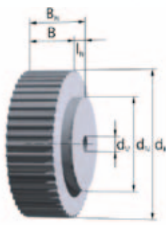
Stock pulleys over z = 44 without flanges
