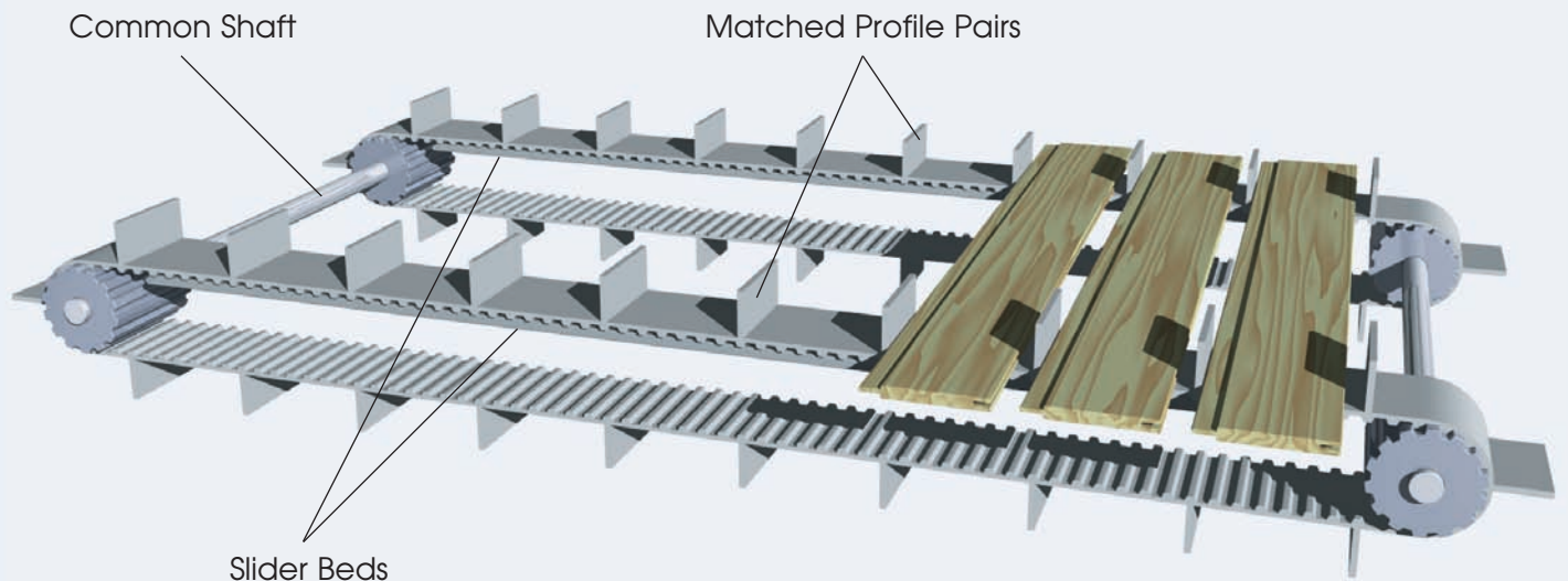
Synchronous Conveyor For Wide Products
