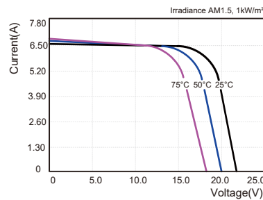
I-V Curves of PV module SY-S120W at various cell temperatures
