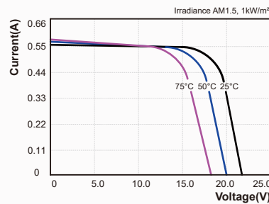
I-V Curves of PV module SY-S10W at various cell temperatures
