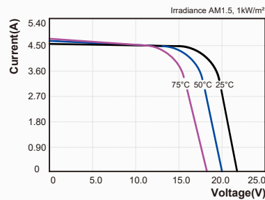
I-V Curves of PV module SY-M80W at various cell temperatures
