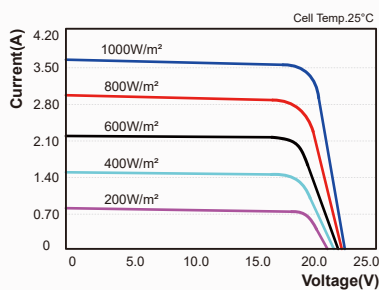
I-V Curves of PV module SY-M60W
