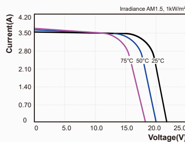
I-V Curves of PV module SY-M60W at various cell temperatures
