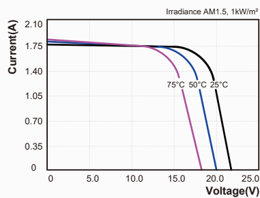
I-V Curves of PV module SY-M30W at various cell temperatures
