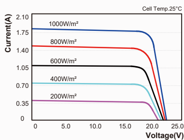
I-V Curves of PV module SY-M30W
