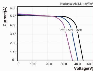
I-V Curves of PV module SY-M200W at various cell temperatures
