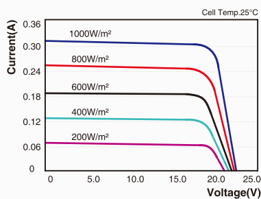
I-V Curves of PV module SY-M05W
