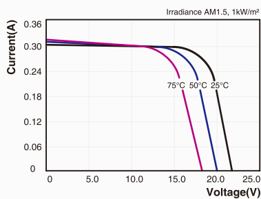
I-V Curves of PV module SY-M05W at various cell temperatures
